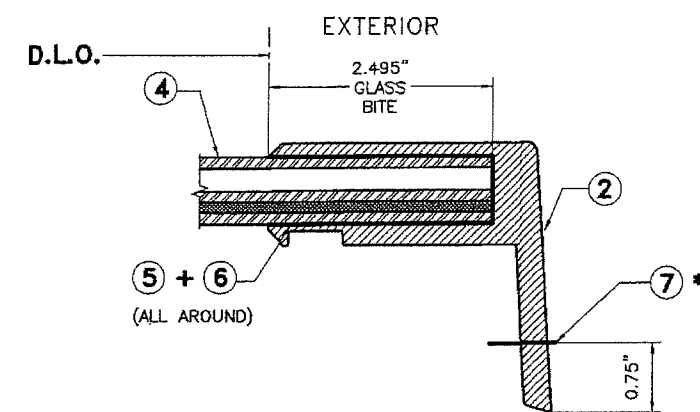
DETAIL "B"
