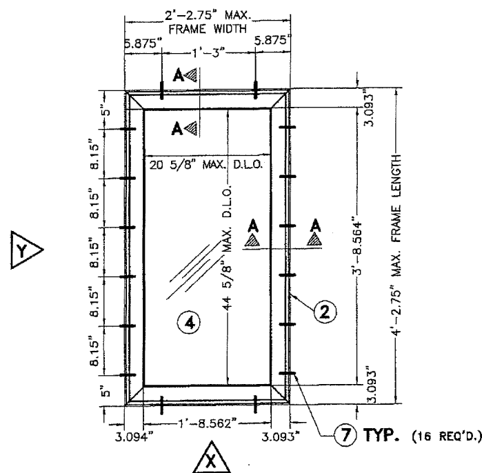
PLAN (EXTERIOR SIDE)
