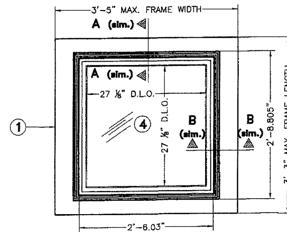
PLAN (INTERIOR SIDE)
