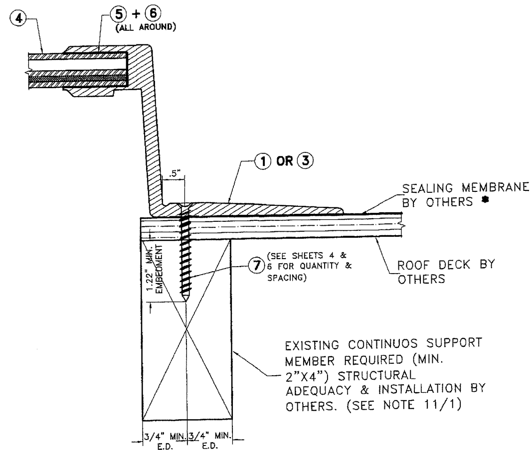
CONNECTION DETAIL FOR FRAME CASES 1 & 3 (SSF)
