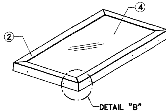
TYPICAL ISOMETRIC
