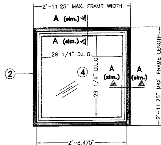
PLAN (INTERIOR SIDE)
