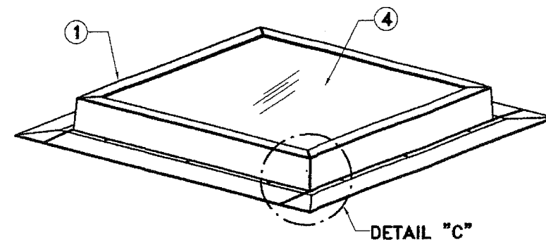
TYPICAL ISOMETRIC
