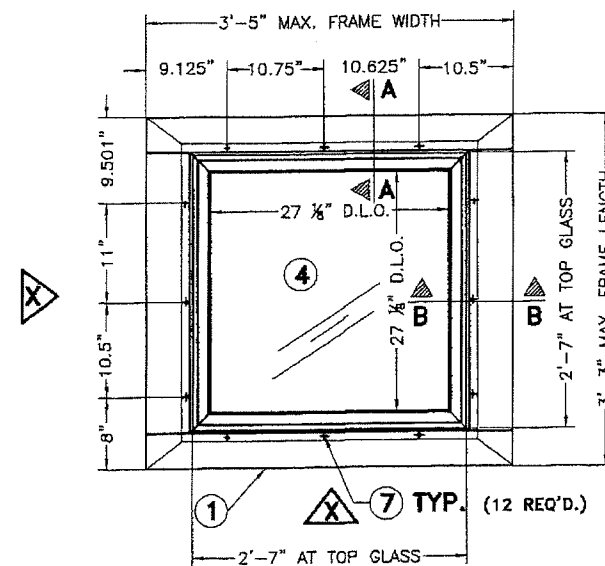
PLAN (EXTERIOR SIDE)
