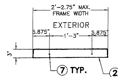
VIEW X
