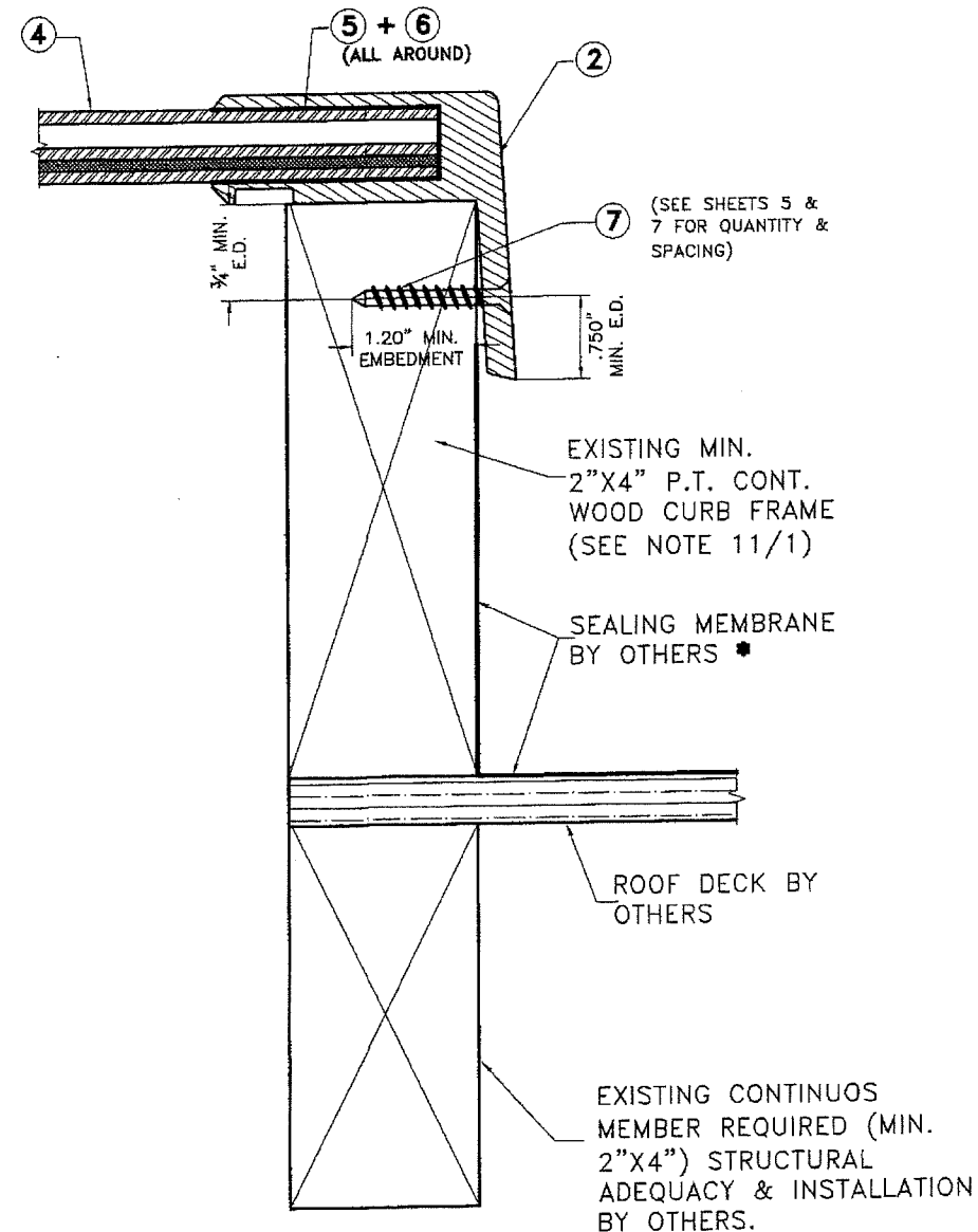
CONNECTION DETAIL FOR FRAME CASES 2 & 4 (CAP)
