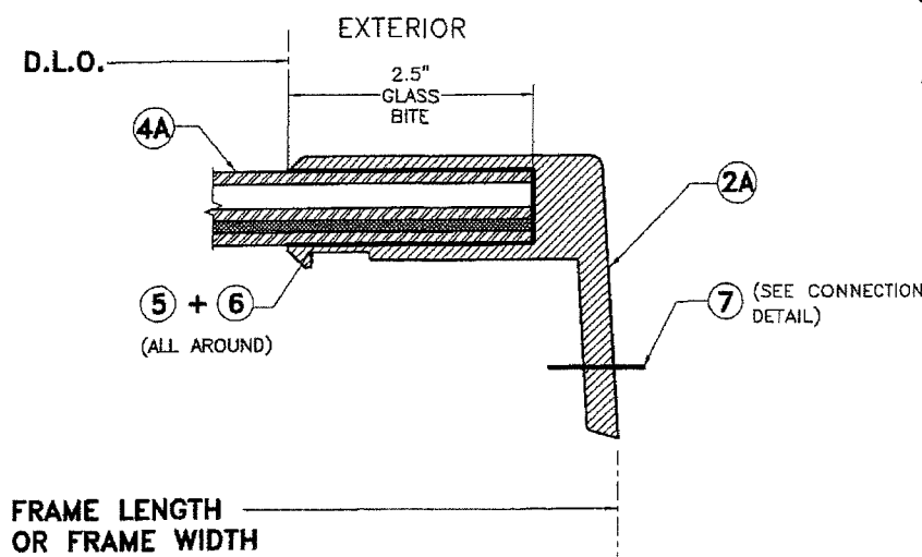
SECTION A-A SCALE: 1/2"=1" GLAZING DETAIL
